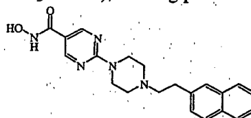
.079 CF 3 COOH compound 7
